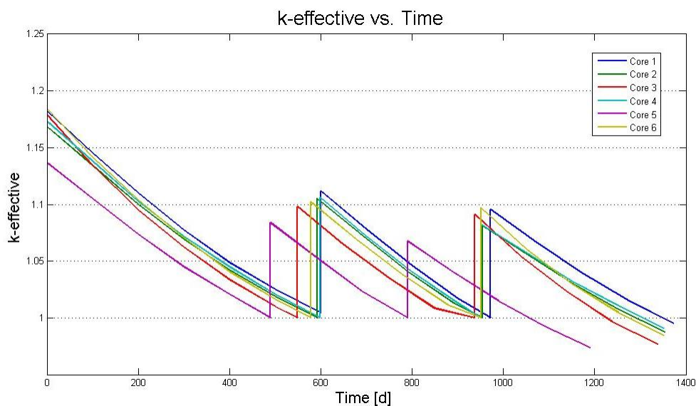
Figure 3.16. k_{eff} vs. Time for Three MCNP Burn Cycles
